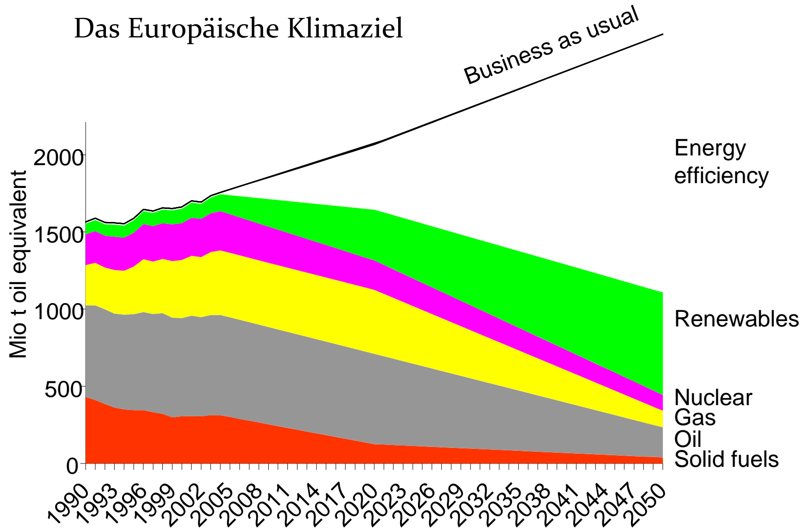
Figure 4.4 Using long-term emissions targets to assess the roles of different technologies over the next four decades (example EU-25).
