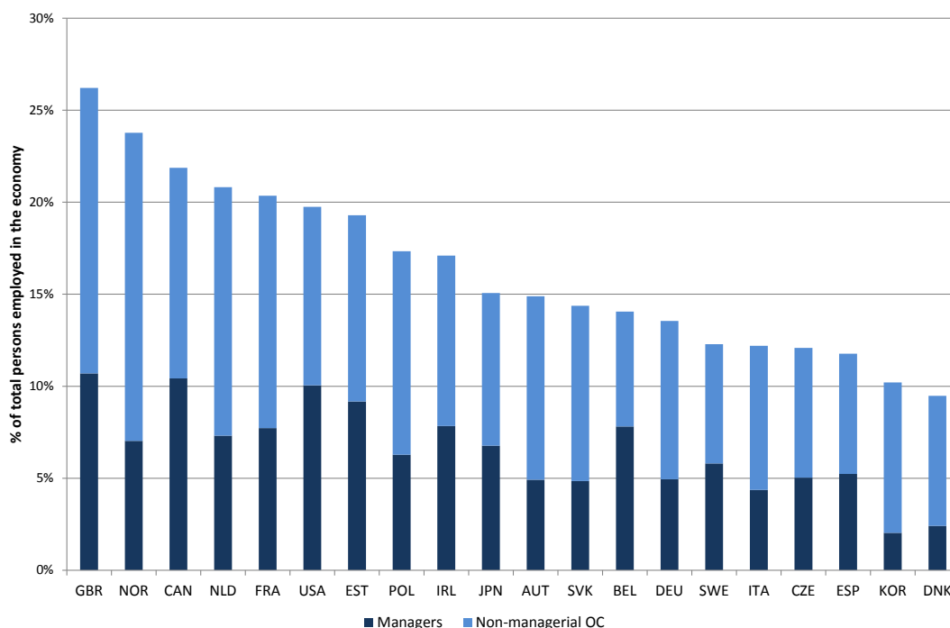
Figure 1. OC-related workers, 2012
