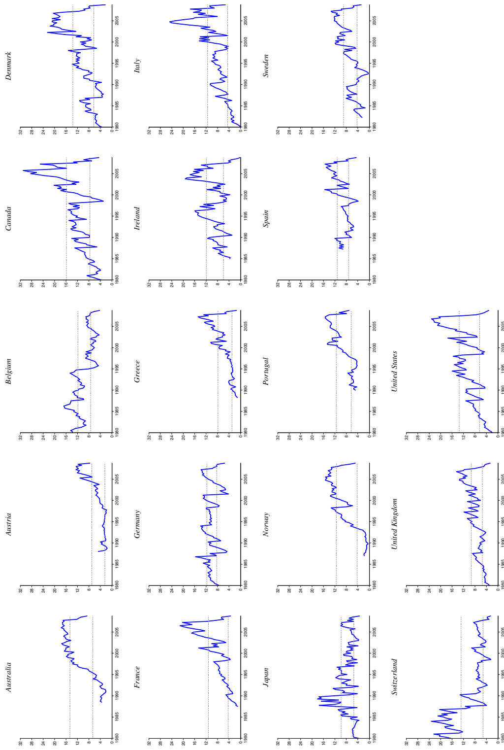
FIG. 1. ESTIMATED DISTANCE-TO-DEFAULTS
