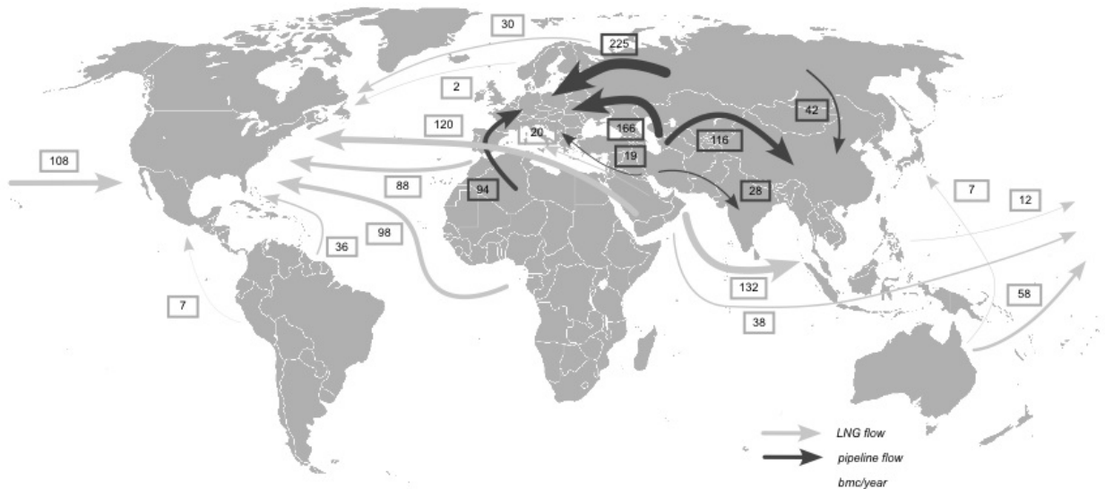
Figure 7: Natural gas flows in 2030 by region; in bcm/y, „in the ground“ scenario
