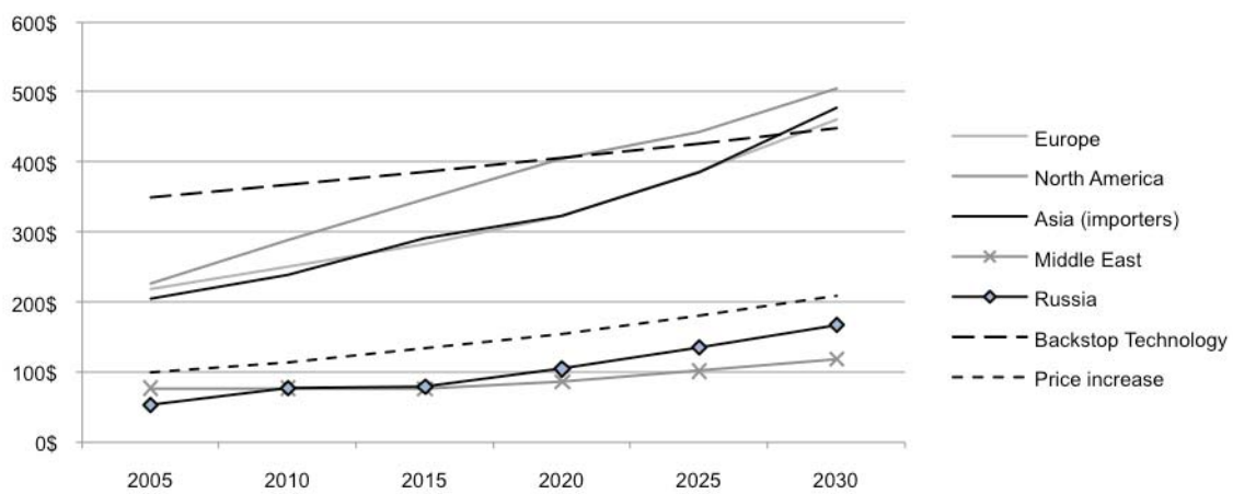
Figure 8: Average wholesale prices (base case), backstop technology costs (post Bali scenario); in $/kcm
