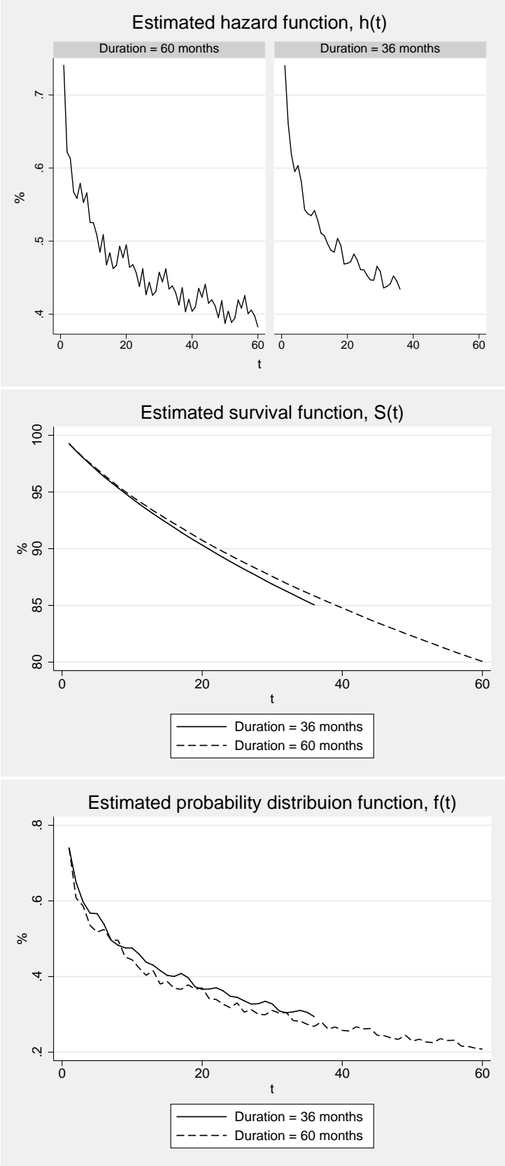
Figure 2: Estimated functions
