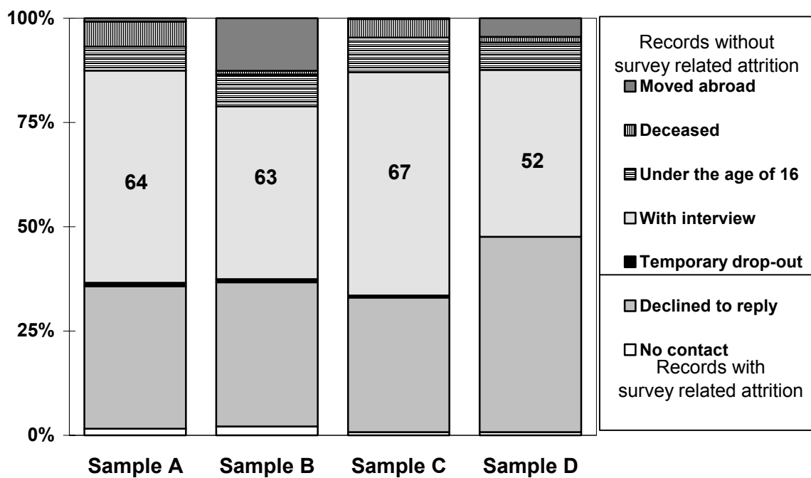
Figure 18: All first wave persons (A, B, C, D). Comparison of the development until wave 10.
