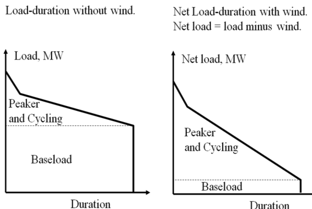
Figure 8. Load-duration and net load-duration.
