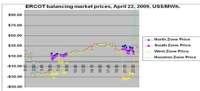
Figure 9. Negative prices throughout ERCOT in early morning. Source: [20].
