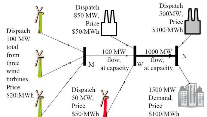
Figure 5. Dispatch and prices with limited transmission.
