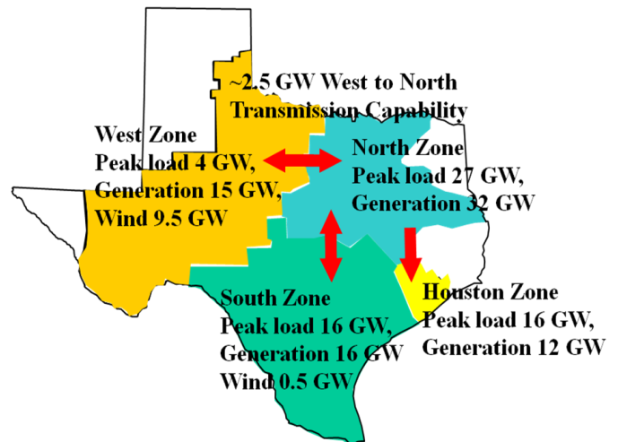
Figure 4. ERCOT zones and approximate peak load and generation capacity levels. Source: Based on [12].
