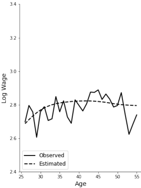
Figure 5: Model fit
