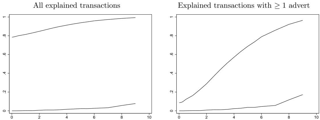
Figure 4: Bounds on the cdf of minimum search cost \underline{s}
